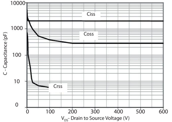
Capacitance
