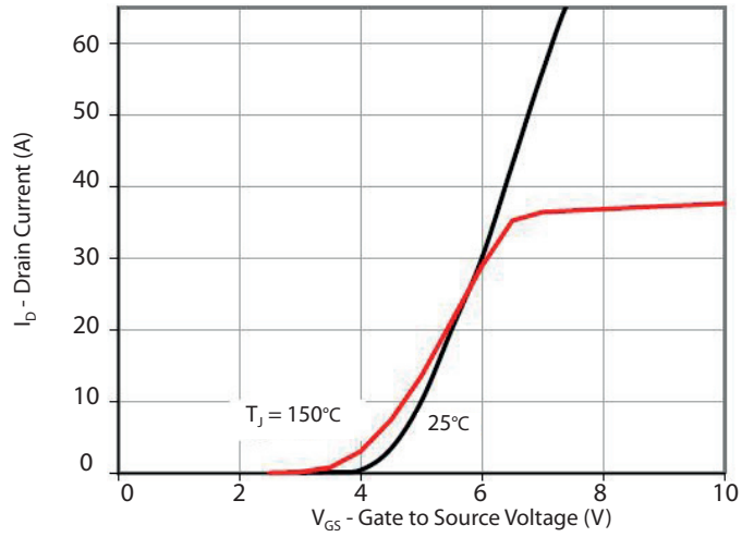
Transfer Characteristics
